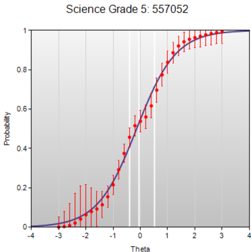
Figure 9-1a. Item Calibration Example Plots (Exemplar)
