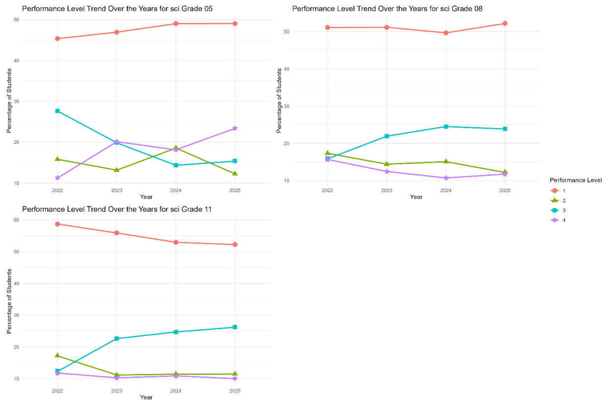
Figure 1-1 Science Student Longitudinal Performance
