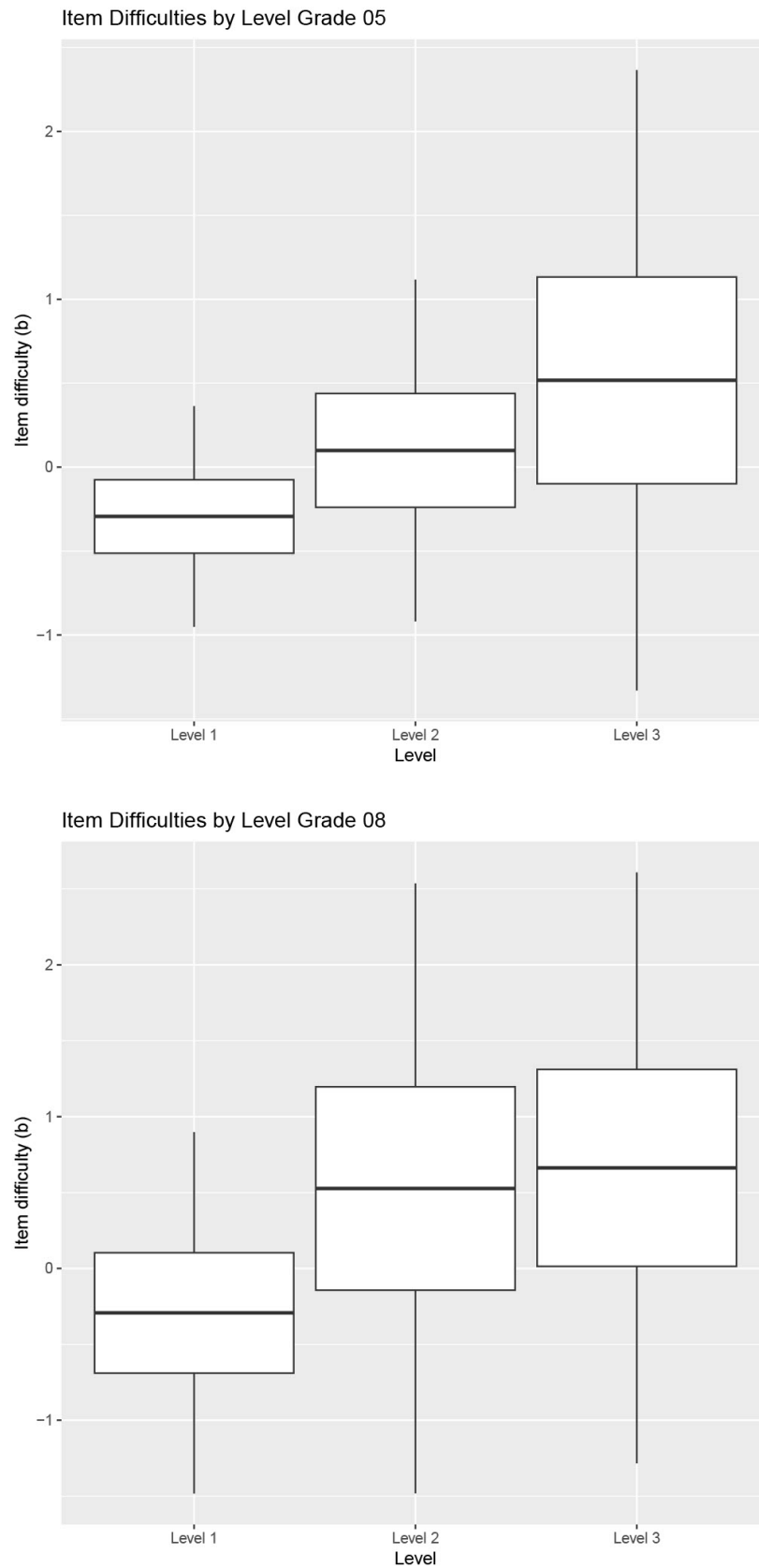
Figure 9-2. Boxplots of IRT Summary Statistics by Grade and Level
