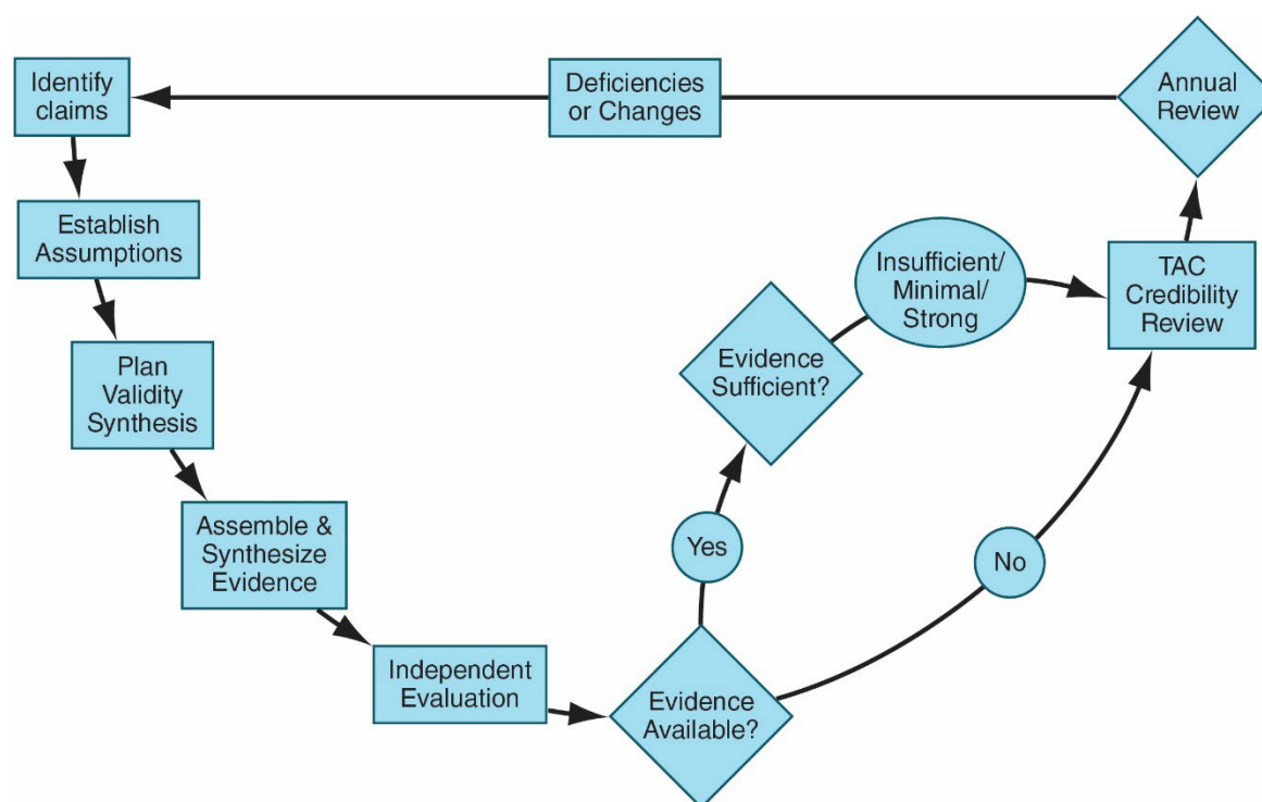
Figure 11-1. MSAA Validation Framework
